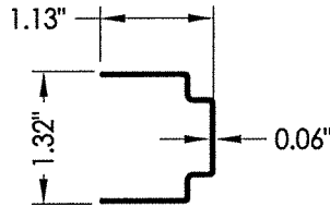
18 LOCK STILE STIFFENER 356-S1552-LR
