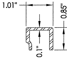
23 REINFORCEMENT 356-A61-B
